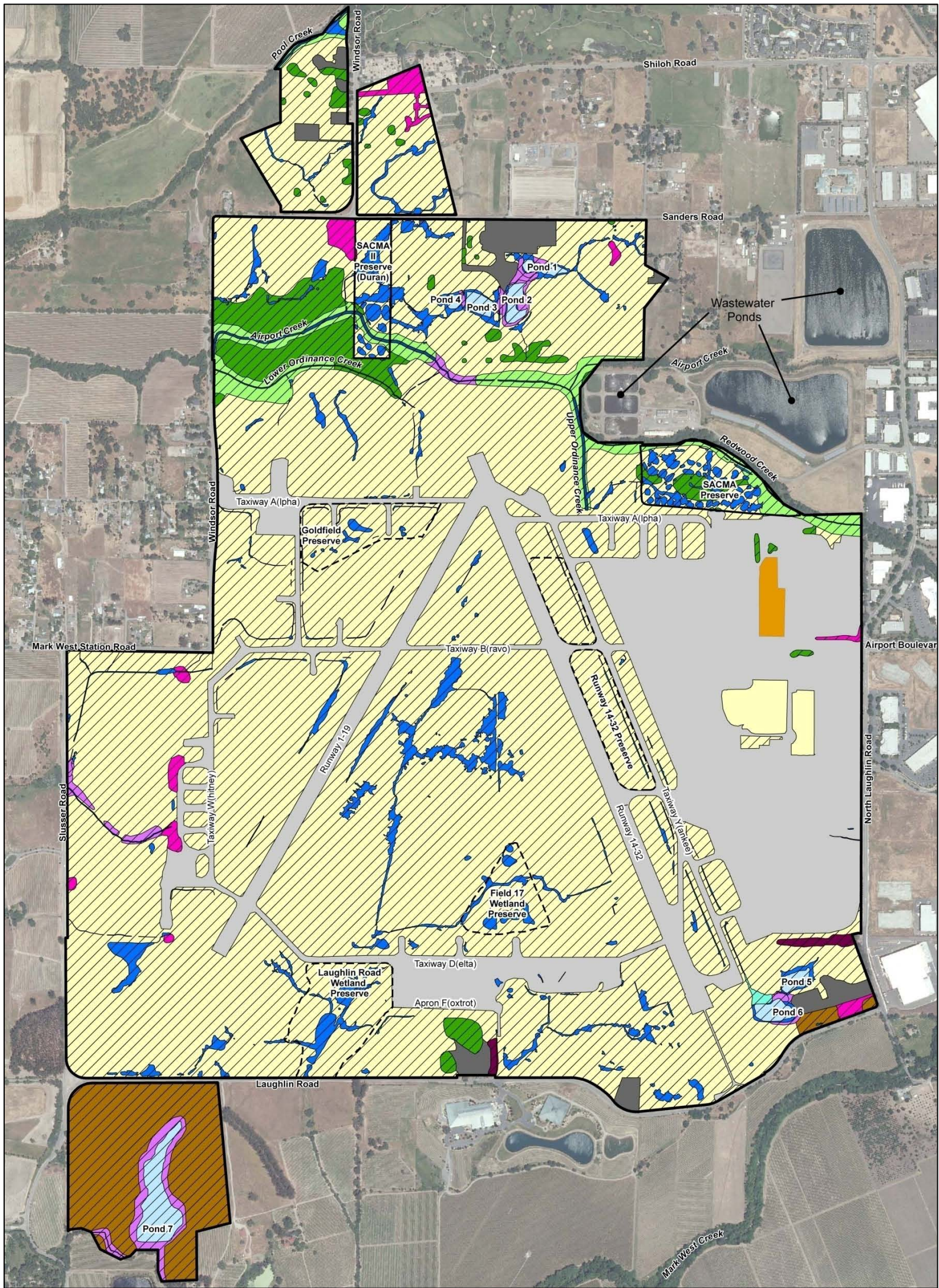
Figure 3.4-6 CALIFORNIA TIGER SALAMANDER SUITABLE HABITAT
