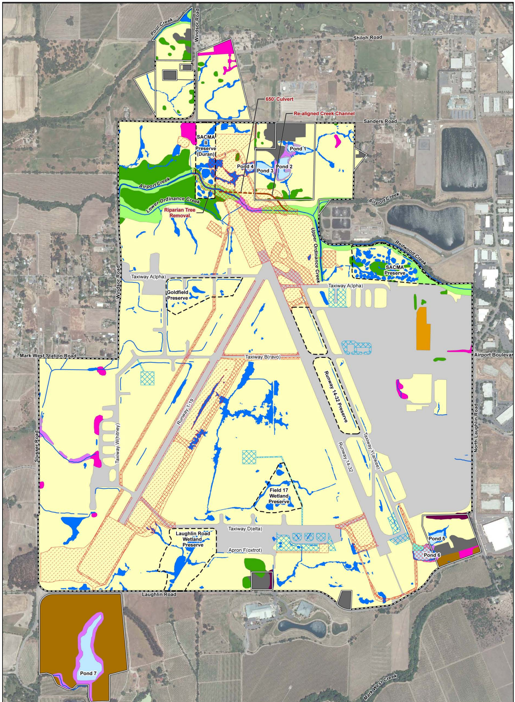
Figure 3.4-1 SHORT-TERM AND LONG-TERM PROJECTS - AIRPORT MASTER PLAN
